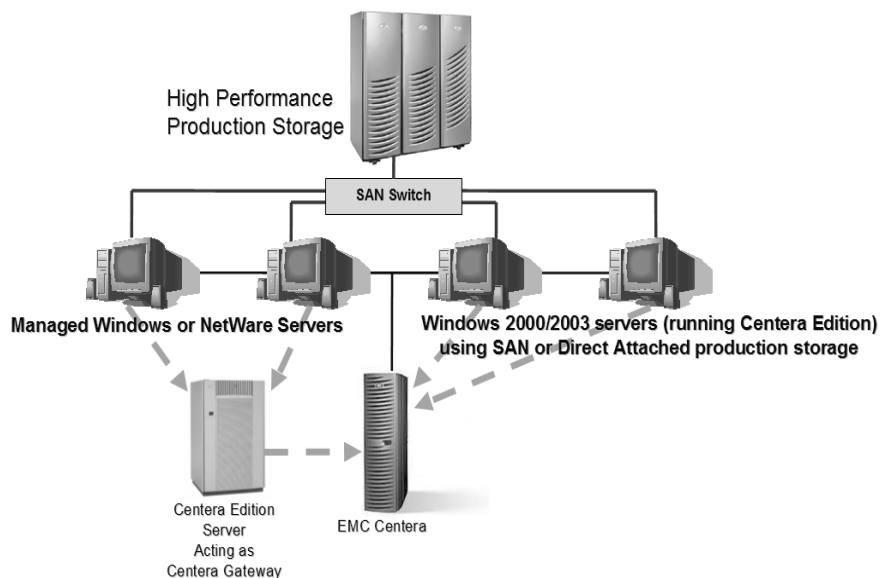
Managed Server HSM – Centera Edition, running on a Windows 2000/2003 server, can manage files directly from its own resources to the Centera. Or, optionally, it can act as a gateway to Centera providing access from multiple NetWare and Windows “managed” servers.
